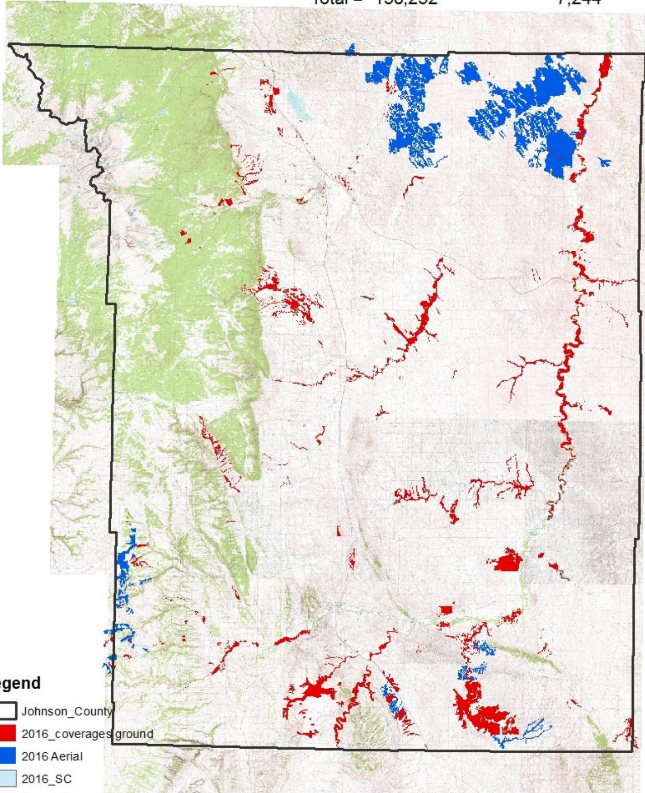
The map shows the acres covered by the District in 2016. 494 application records were processed during the year. The following graphs show the percentage based on acres of applicatons and program dollars.
